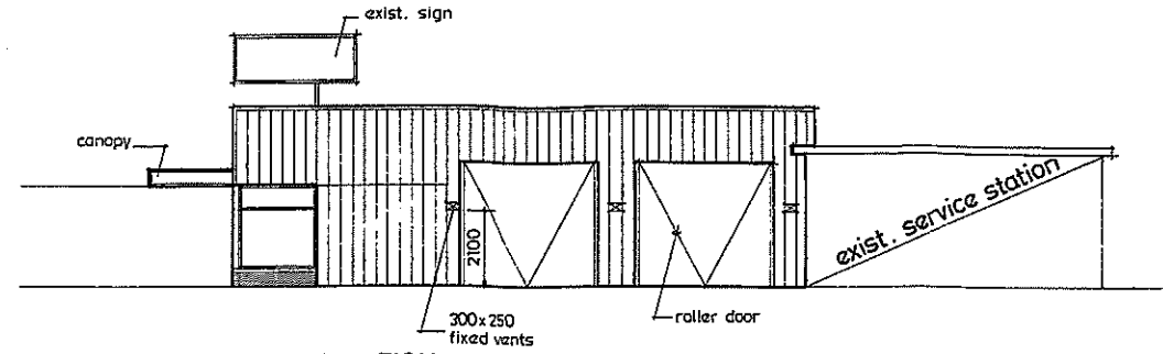
EAST ELEVATION
