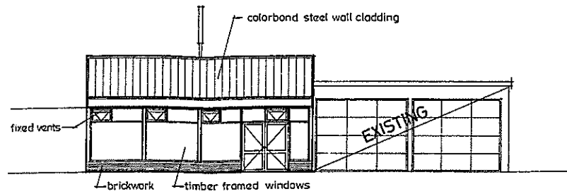
SOUTH ELEVATION
